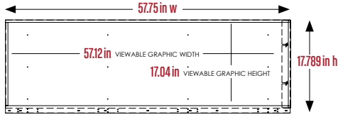
OPTIONAL NON-ILLUMINATED TOPPER
