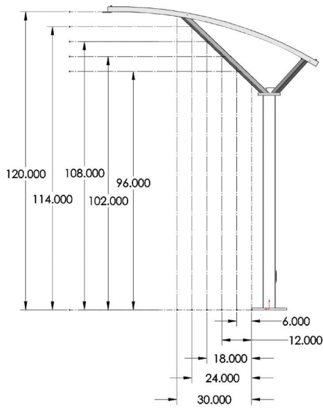
CLEARANCE HEIGHT
